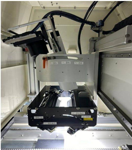
SN Visual machine Camera
